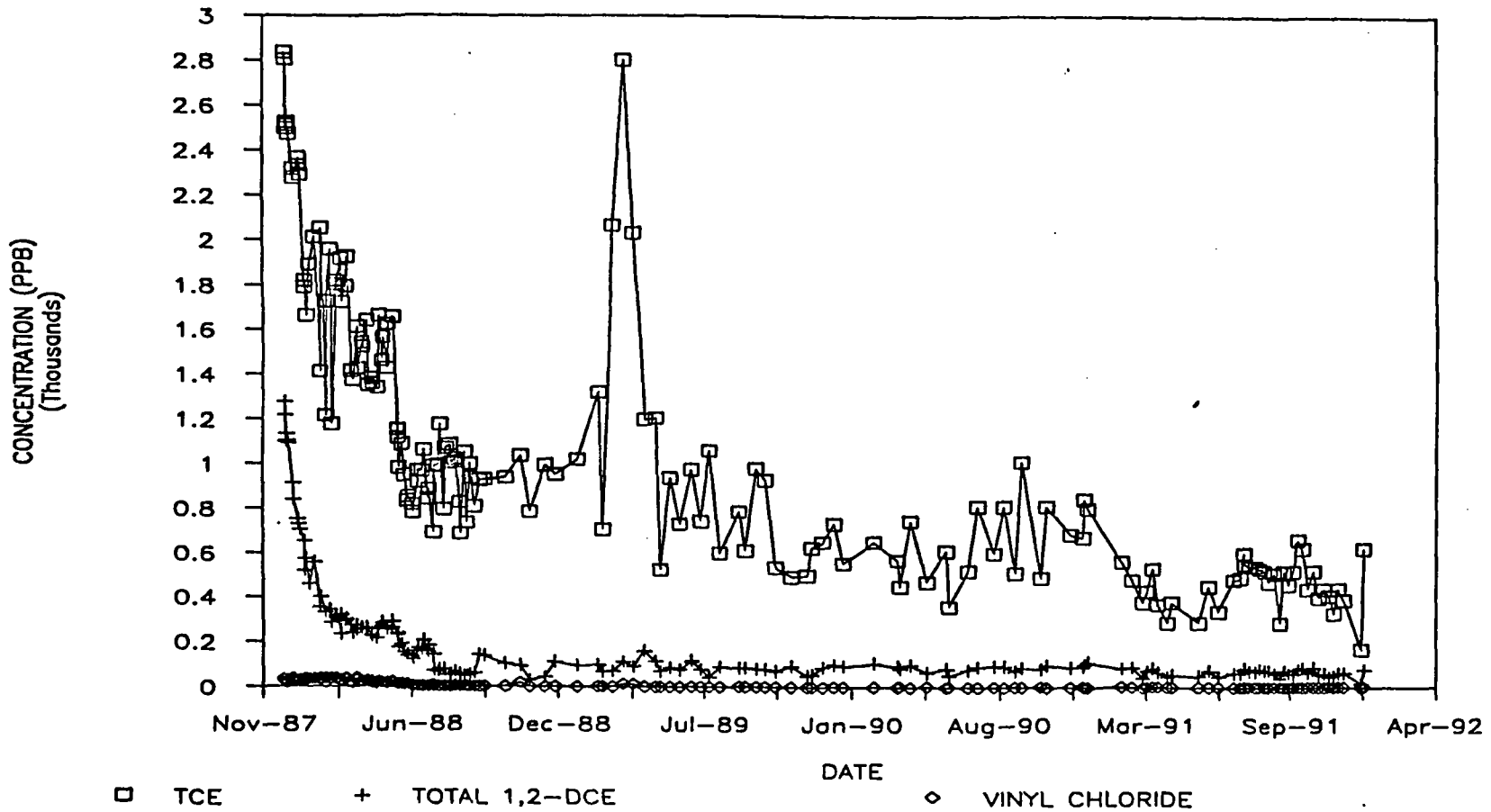
FIGURE 7-3 AIR STRIPPER INFLUENT CONCENTRATION DECEMBER 1987 - DECEMBER 1991 DES MOINES SOUTH AREA SOURCE CONTROL PROJECT ECKENFELDER INC. Nashville, Tennessee Mahwah, New Jersey
